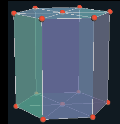
▲ The mineral weissbergite, TlSbS_2 .
